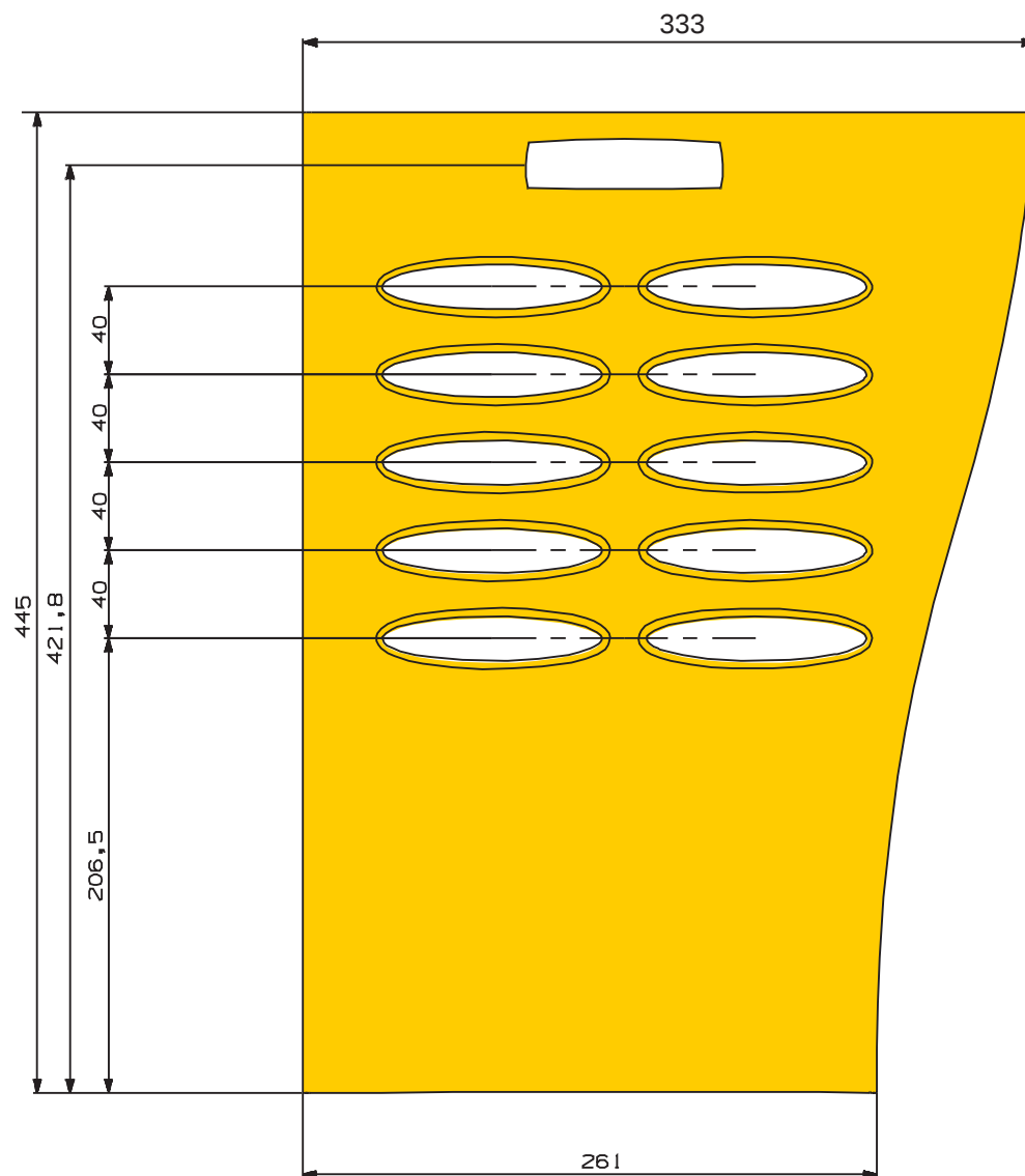
Pannello frontale Frontal panel
